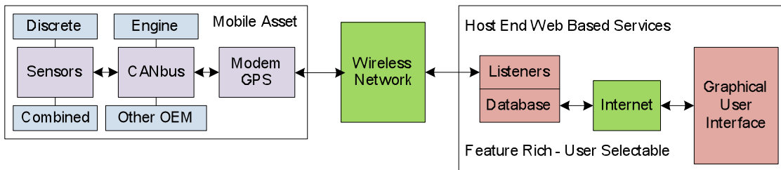
Figure 2: Block Diagram of On-board Equipment & Host End Services
